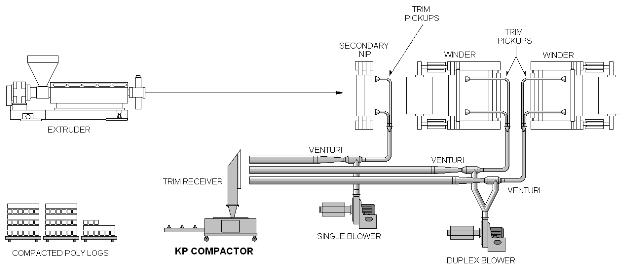
JTW inducer trim conveying systems can be integrated with in-line trim recycling, repelletizing or compacting systems, as shown.
